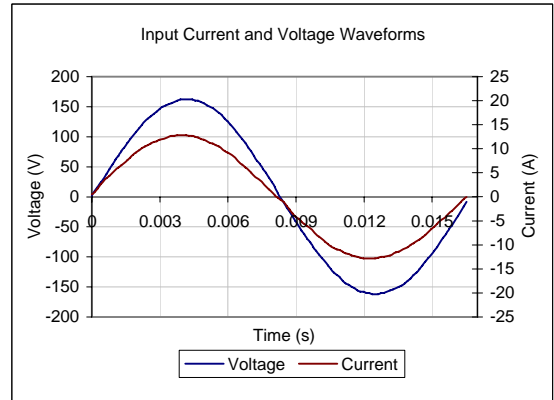
Input AC Current Waveform (ITHD = 2.88%, 50% Load)
