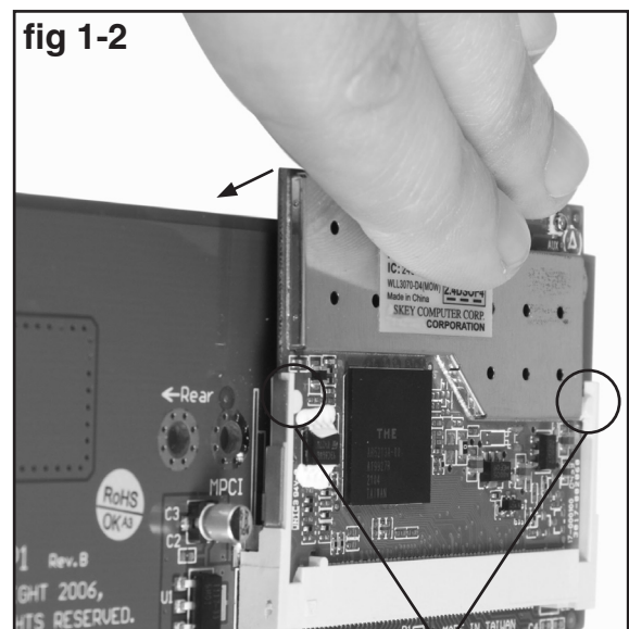
Retaining Notches
