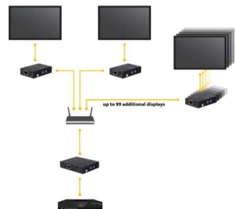
Point-to-Multipoint (Unicast)
